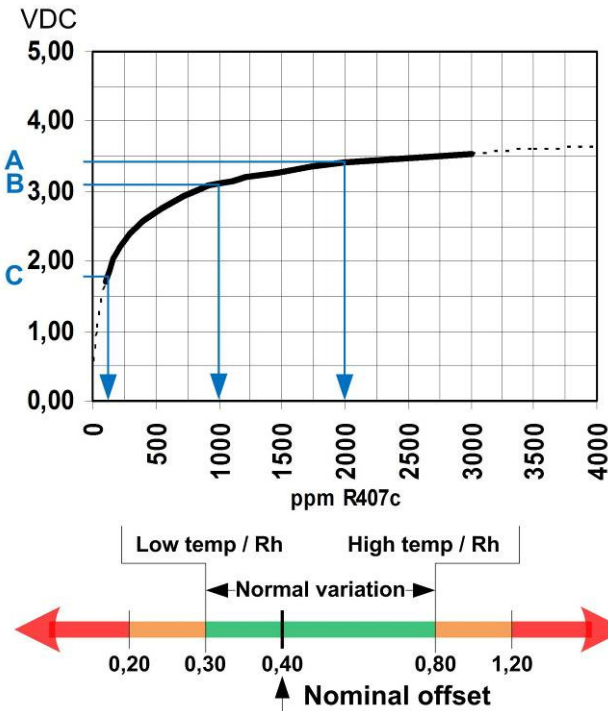
R407c - Range: 0 – 4000 ppm Part number: SEN004
