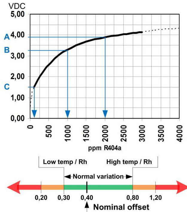
R404a / R507c - Range: 0 – 4000 ppm Part number: SEN004
