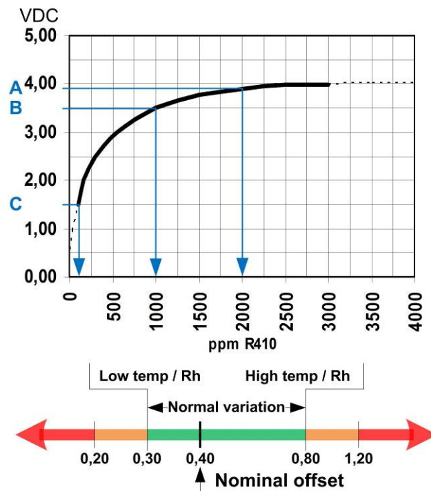
R410A - Range: 0 – 4000 ppm Part number: SEN004
