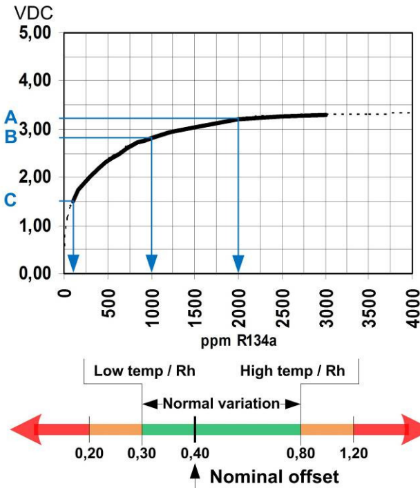
R134a - Range: 0 – 4000 ppm Part number: SEN004
